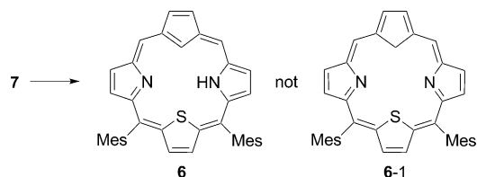
Scheme 4. Oxidation of 7 : [\text{D}_6]\text{chloroform} , DDQ (1 equiv) dissolved in [\text{D}_6]\text{benzene} , RT, 20 min.
